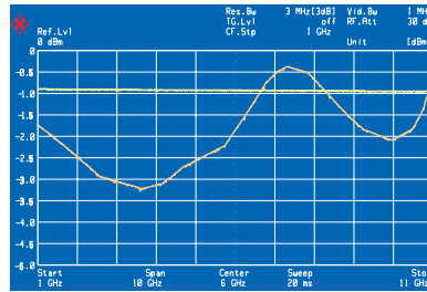
FIG 6: Output level with frequency response correction ON (yellow curve) and OFF (orange curve)
