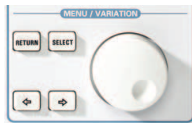
FIG 10: General settings and menu selection with spinwheel, RETURN, SELECT and arrow keys
