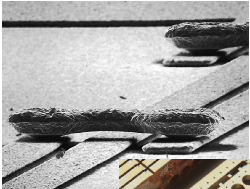
Airbridges is an ideal technique for implementing PCB crossovers with excellent high-frequency characteristics. The photo above has been taken with a scanning electron microscope and shows such an airbridge which is only 0.05 mm long.
